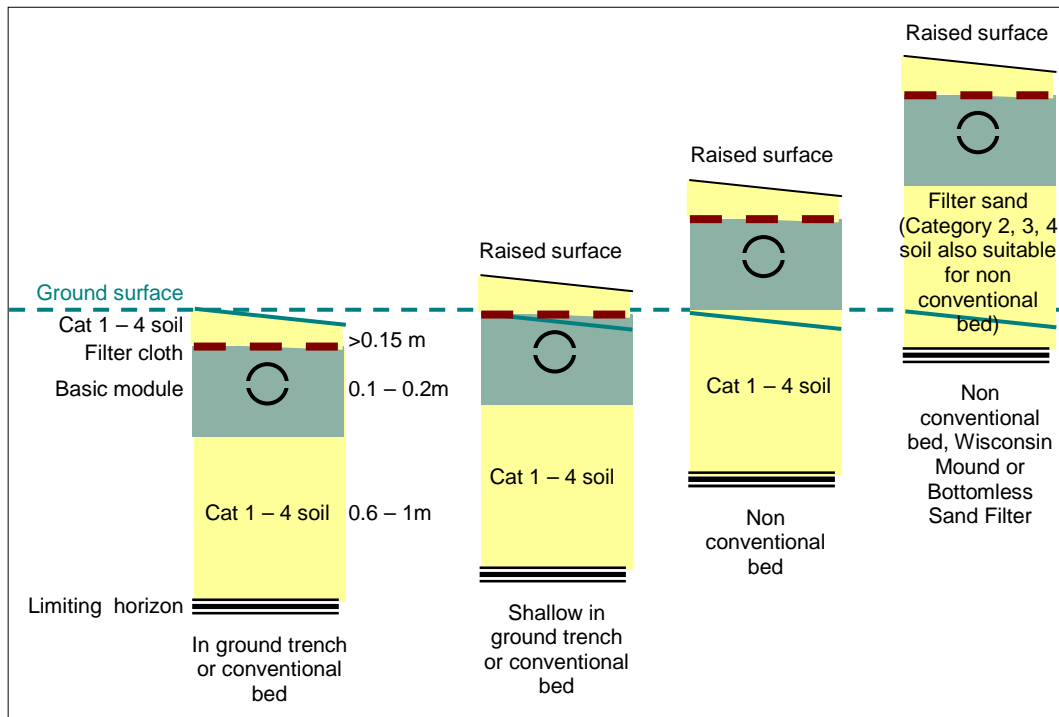
Figure 5. Cross sections of four wastewater disposal systems in relation to ground surface and the depth to a limiting horizon. Adapted from Converse and Tyler (2000) and Cromer (2004)
