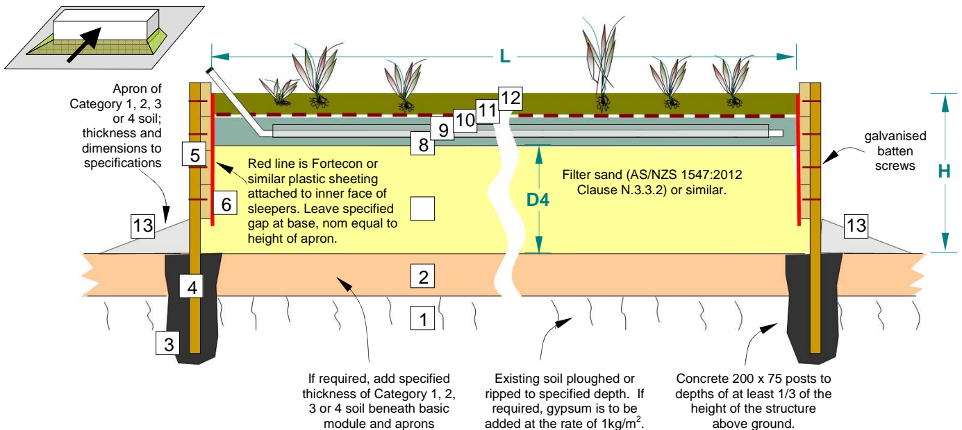
Figure 9b. Generalised side to side section of a typical BSF along a contour. Refer to Table 1 for more information for, and typical dimensions of, the numbered and lettered features. Also use Table 1 to insert site-specific dimensions to assist in tendering for and pricing BSFs.
