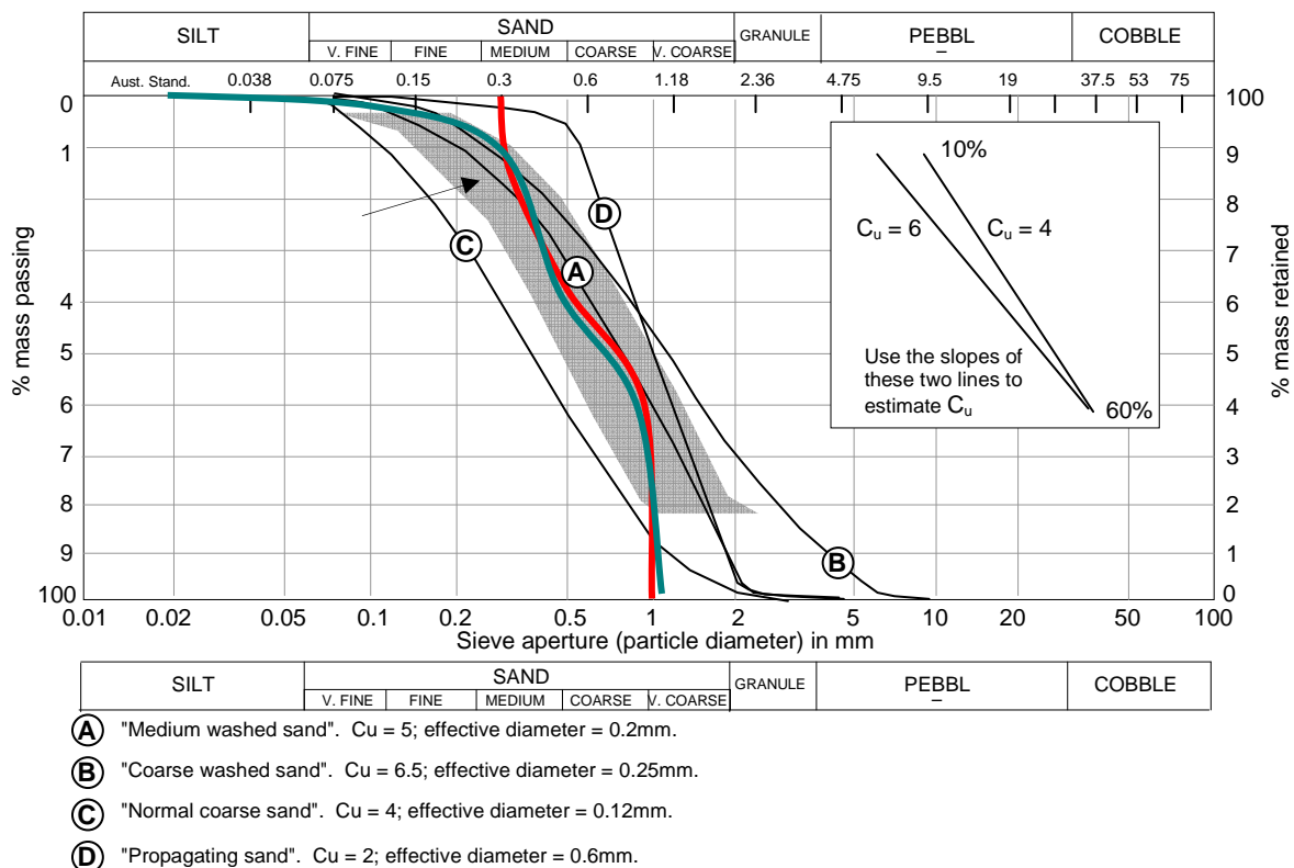
Figure 6. Grain size curves A – D for some Tasmanian commercial screened sand materials (modified from Cromer, 2004). The grey envelope approximately includes the range of sand specifications suggested by Converse and Tyler (2000) for a Wisconsin Mound. The red and green lines are two of a series of curves that comply with Clause N3.3.2 of AS/NZS1547:2012; in both cases, the C_u is about 3.3.
