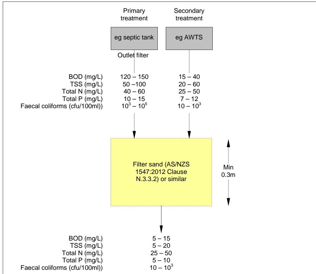
Figure 7. Approximate treatment efficiencies of filter sand
