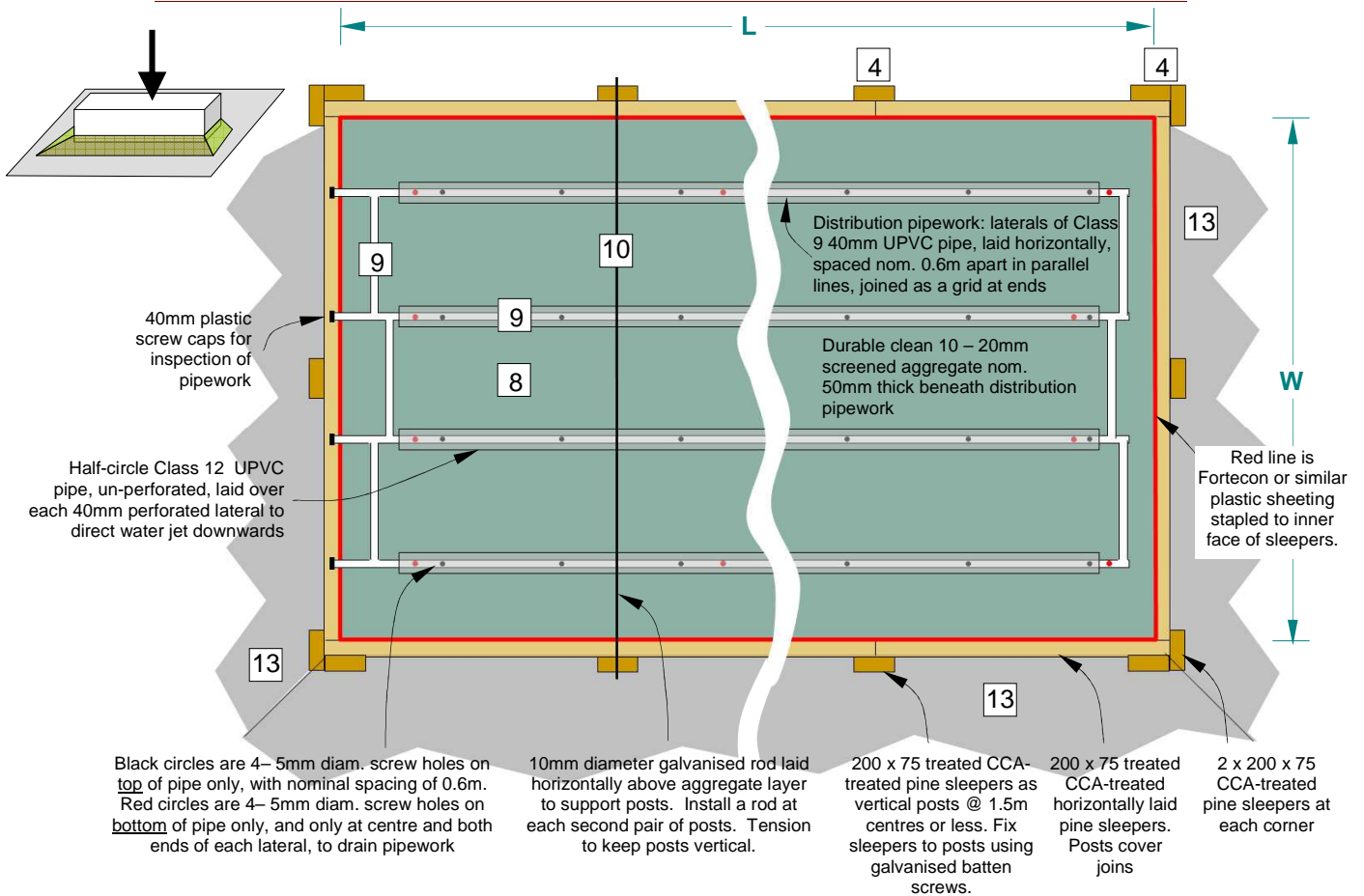
Figure 9a. Generalised plan of a typical BSF. Refer to Table 1 for more information for, and typical dimensions of, the numbered and lettered features. Also use Table 1 to insert site-specific dimensions to assist in tendering and pricing BSFs.
