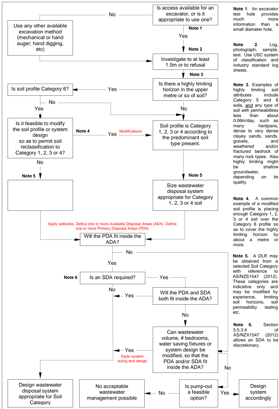
Figure 4 Flow chart for on-site wastewater assessment. Elements of this flow sheet have been influenced by Schedule 12 of Sorell Council's Planning Scheme 1993 (amended 10 Aug 2011). Other approaches may be acceptable.
