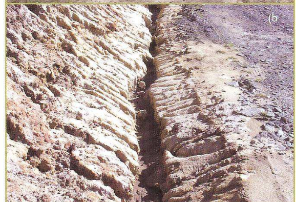
Figure 6 (a). Tunnel erosion resulting from construction of a culvert in dispersive clay (b). Tunnel erosion caused by installation of optical fibre cable in dispersive soil.
